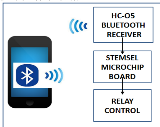
Figure.1 Architecture of Automation Project
