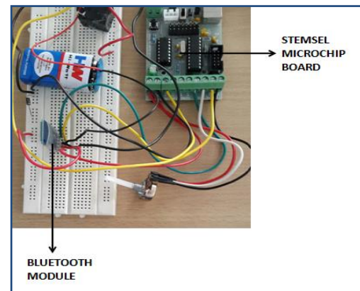
Figure.2 Bluetooth Automation Prototype Using STEMSEL Microchip Board
